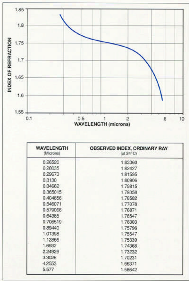
Figura 1. Observed Indices of Refraction for Sapphire versus Wavelength 1
